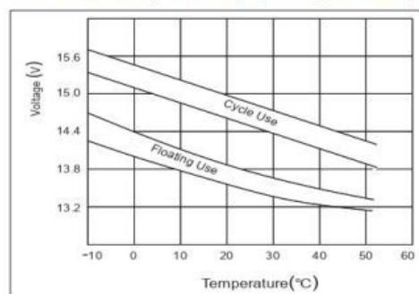
► The Relationship for Charging Voltage and Temperature
