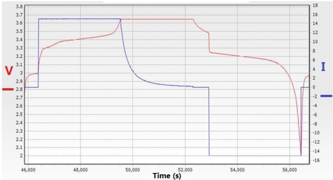
40152S discharging and charging curves at discharging rate of 1C:
