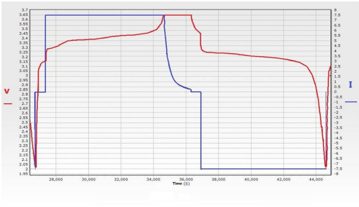
40152S discharging and charging curves at 0.5C:
