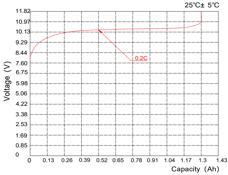
charge curve
